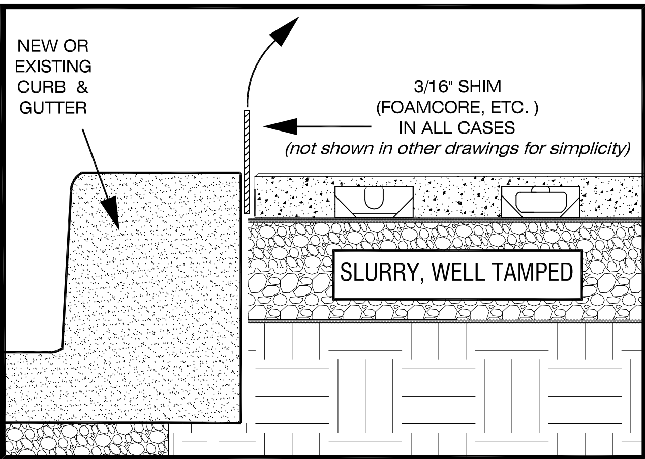
3. NEW OR EXISTING CURB: SUBSTRATE PACKED WITH SLURRY TO SUPPORT PAVERS
