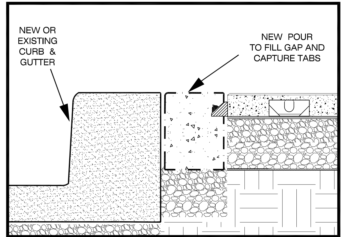
4. NEW OR EXISTING CURB: PAVERS W/ TABS OR RESTRAINTS. AS CONDITIONS REQUIRE. NARROW FILLER OF NEW POUR BETW CURB AND PAVER
