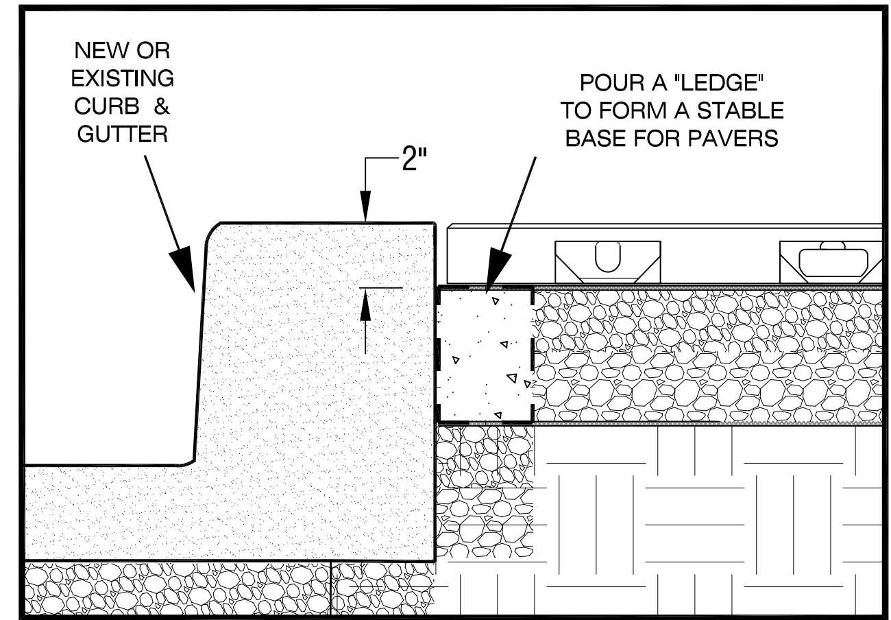
2. NEW CONCRETE SUPPORT SHELF KEEPS PAVER AND CURB HEIGHT ALIGNED
